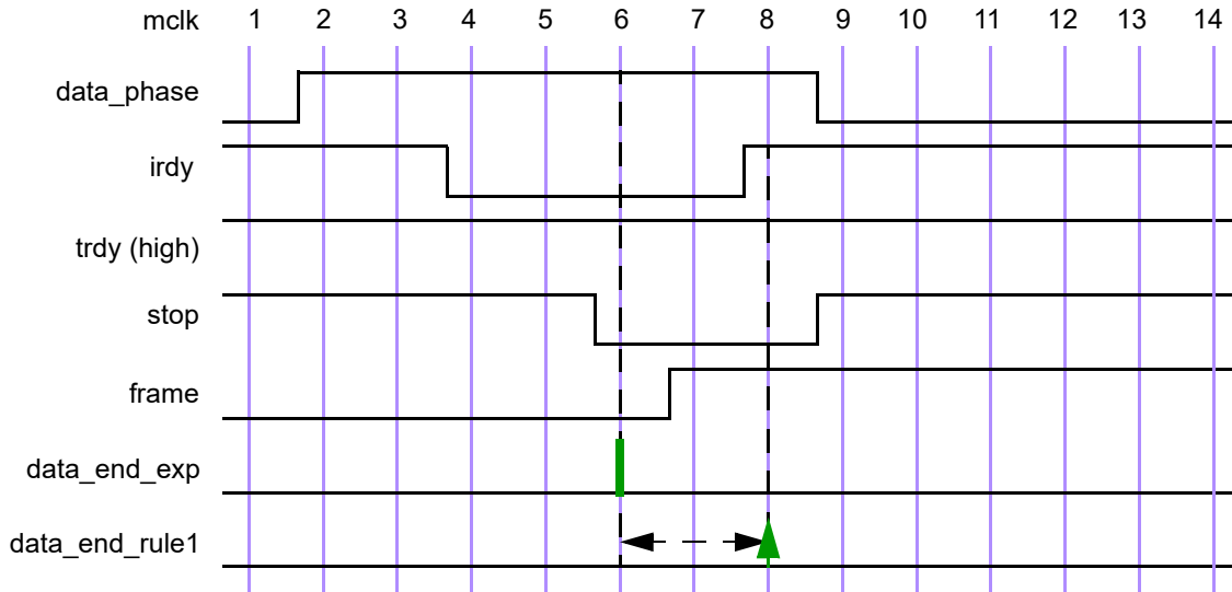
Figure 16-15—Conditional sequences
